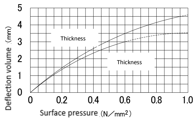
Graph-1 Surface pressure and deflection volume characteristics of Anti-Vibration Pad GPC.
