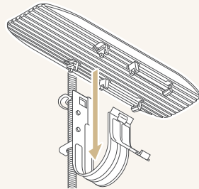
Slide SR-HG to the bottom of SUPERLOCK by passing the hinge part of SUPERLOCK between two nails on the back side of SR-HG.
