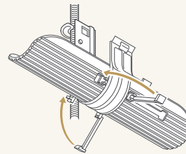
Close lid of SUPERLOCK after installation of piping.
