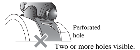
(Figure 2-3) Bad example (The tightening is loose.)
